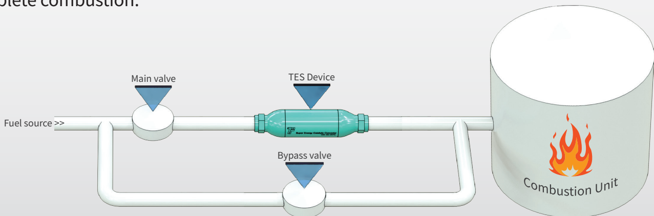
Figure (2): Typical installation arrangement with bypass
