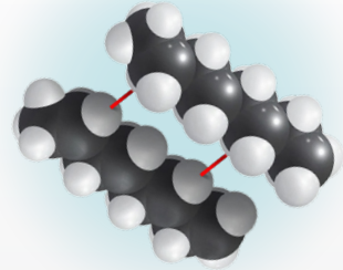
Figure (1) : Intermolecular forces
